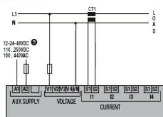
Single-phase
