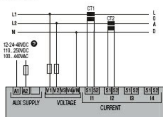
Two-phase
