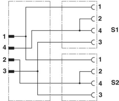
Wiring diagram
