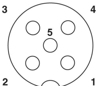
Wiring diagram
