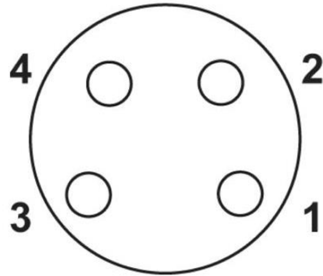
Wiring diagram
