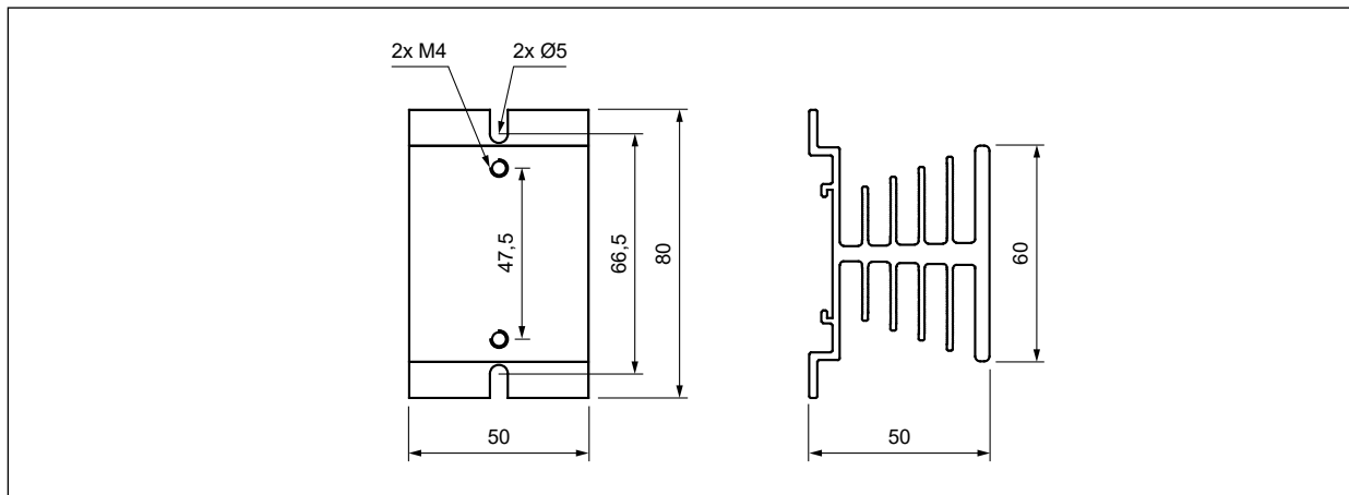
Heatsink RH21
