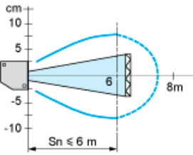
With reflector XU5C50
