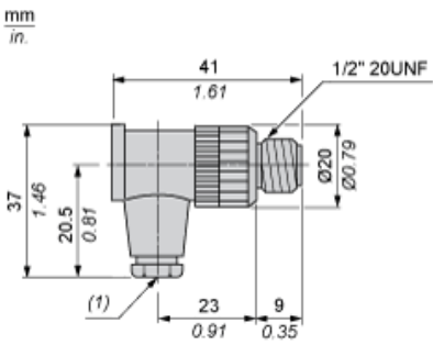
(1) Cable gland : no. 7 plastic (Pg 7)
