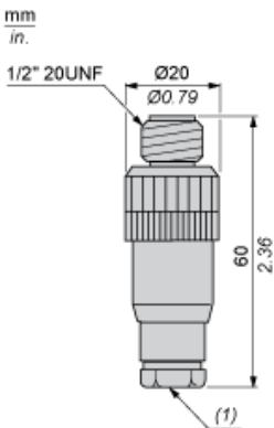
(1) Cable gland : no. 7 plastic (Pg 7)
