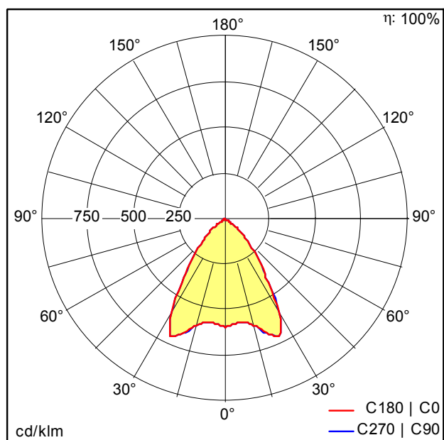
D43023AA_MIRL_A_LED2800-840_Q600_EVG_WH.Idt
