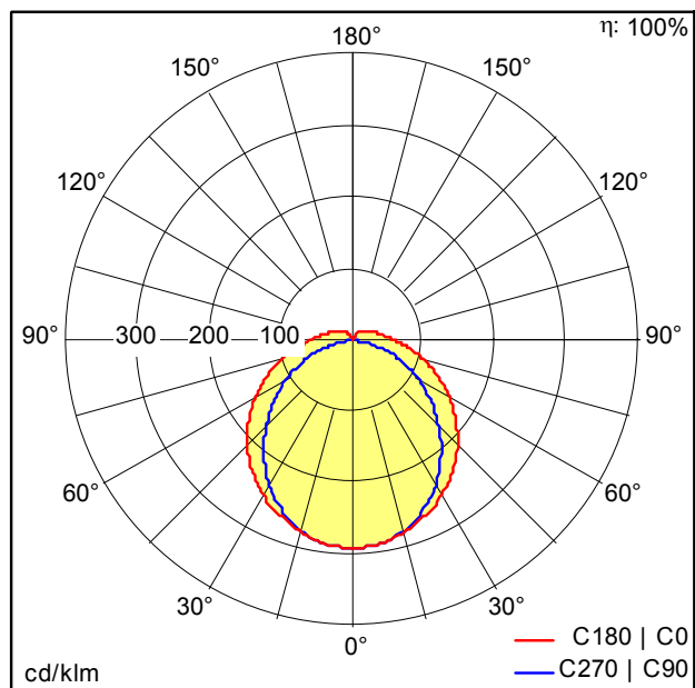
D44080AA_TECTON_B_BASIC_LED5200-840_L1522_LDE_WH.Idt
