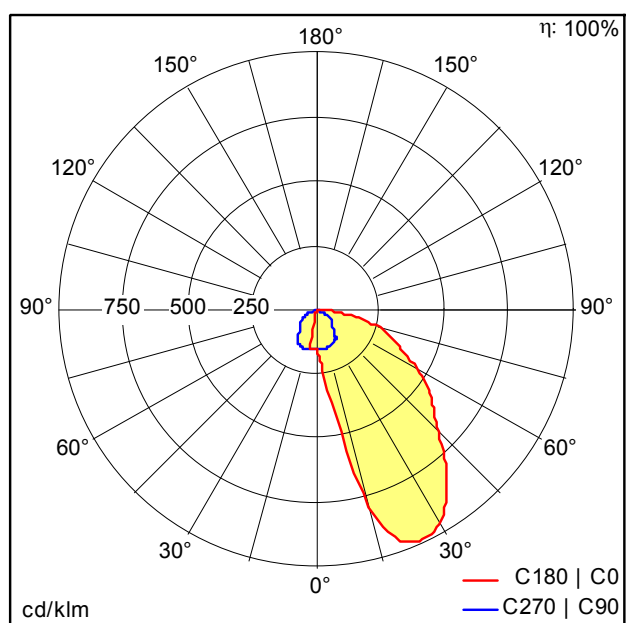
D34983AA_TECTON_C_LED5200-830_L1000_WW_LDE_WH.Idt
