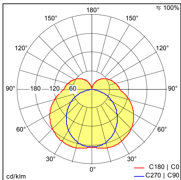
D39715AA_LINARIA_LED3000-830_L1208_PM_WH.Idt
