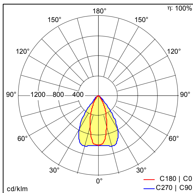
D43181AA_CR2_M17k-840_PC_NB_LDO_WH.Idt
