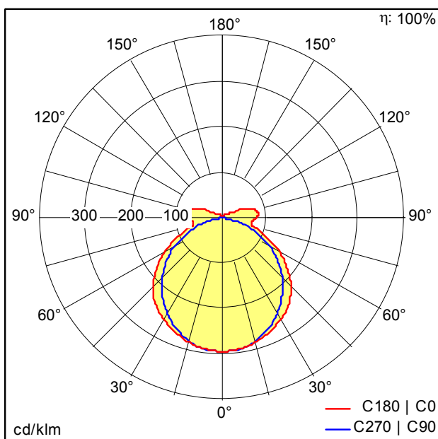
D42468AA_AMP_L_6400-840_CH_MB_LDO.idt
