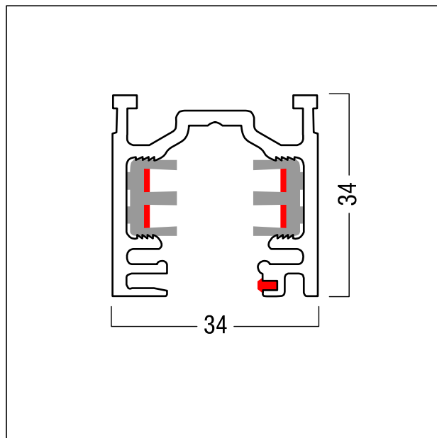
ZS_ST5_M_Normalprofil3PH.wmf
