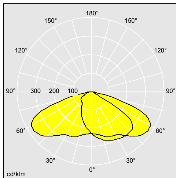
TL_IP24L50WR740.Idt
