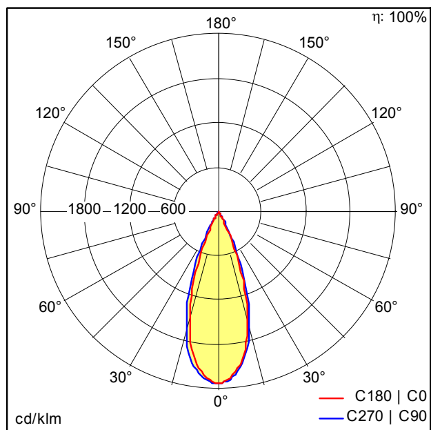
TE_LILY_LED_SPOT_IP44_38_68_850_930.ltd
