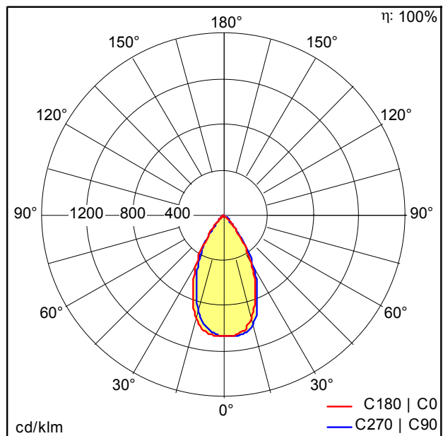
TE_LILY_LED_SPOT_IP44_60_68_600_930.Idt
