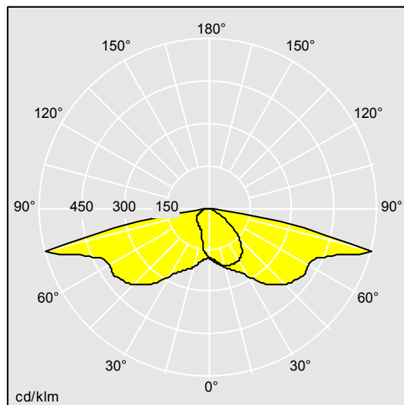
TL_CQS36L70WS740.ltd
