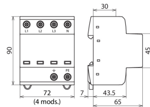
Dimension drawing DSH TNS 255
