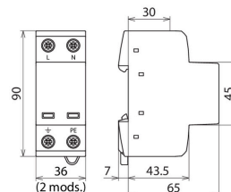
Dimension drawing DSH TT 2P 255
