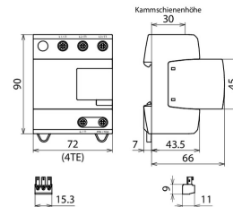
Dimension drawing DV M2 TNC 255 FM
