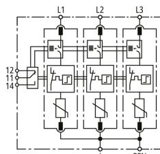
Basic circuit diagram DG M TNC ACI 275 FM
