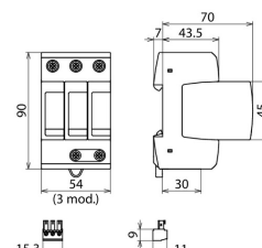
Dimension drawing DG M TNC ACI 275 FM
