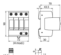
Dimension drawing DG M TT ACI 275 FM
