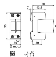
Dimension drawing DG M TN ACI 275 FM
