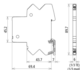
Dimension drawing BCO CL2 BD 12
