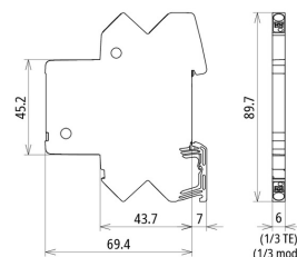
Dimension drawing BCO CL2 BD 24
