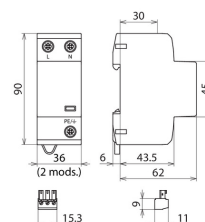
Dimension drawing DSH B TN 255 FM
