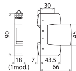
Dimension drawing DR M 2P 255 SN1802
