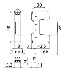
Dimension drawing DR M 2P 255 SN1803FM
