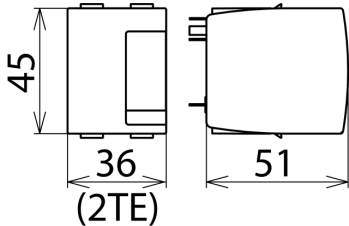
Dimension drawing DR MOD 4P 255 SN1871
