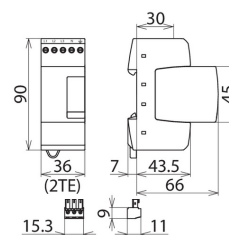
Dimension drawing DR M 4P 255 SN1872 FM
