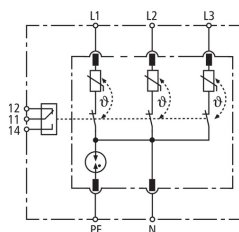
Basic circuit diagram DR M 4P 255 SN1872 FM
