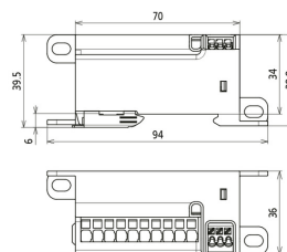
Dimension drawing DCOR 3P TT 275 FM
