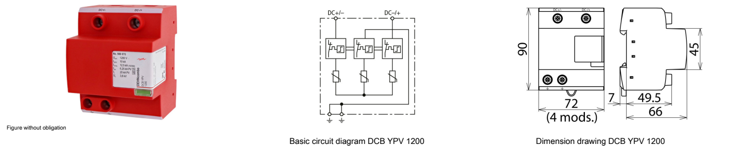
Combined lightning current and surge arrester for use in photovoltaic power supply systems up to 1200 V d.c.
