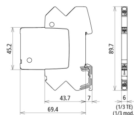
Dimension drawing BCO ML2 BE 24
