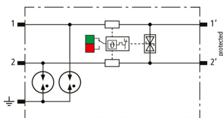
Basic circuit diagram BCO CL2 BD HF 5
