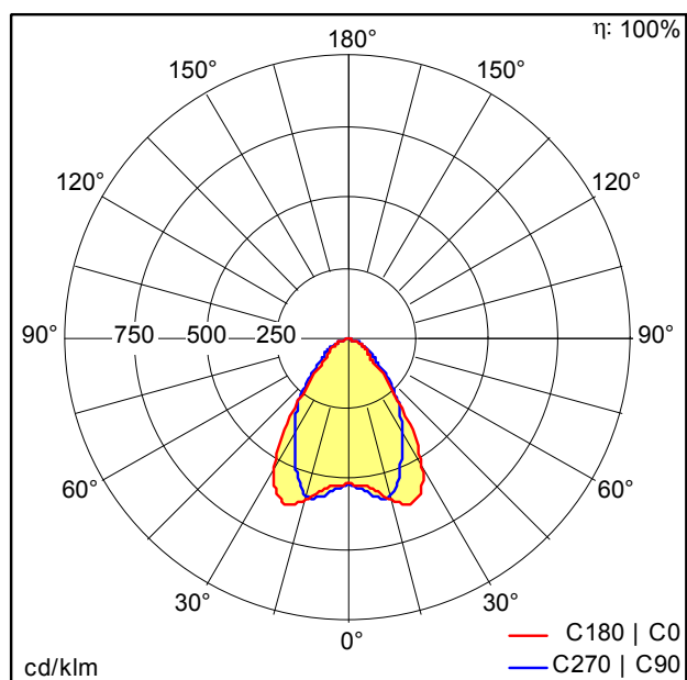
D35001AA_TECTON_C_LED8000-830_L1500_WB_LDE_WH.Idt
