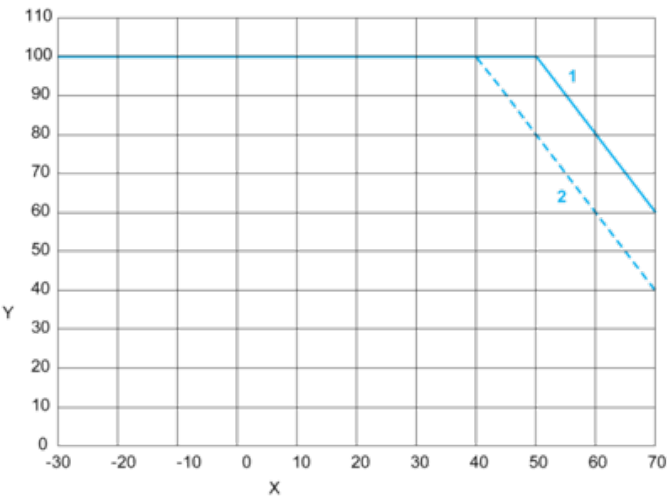
Mounting Position A, B and G
