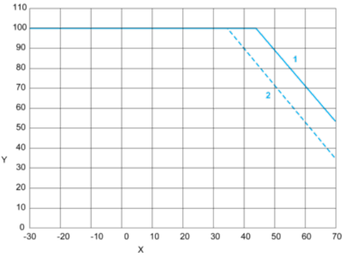
Mounting Position C
