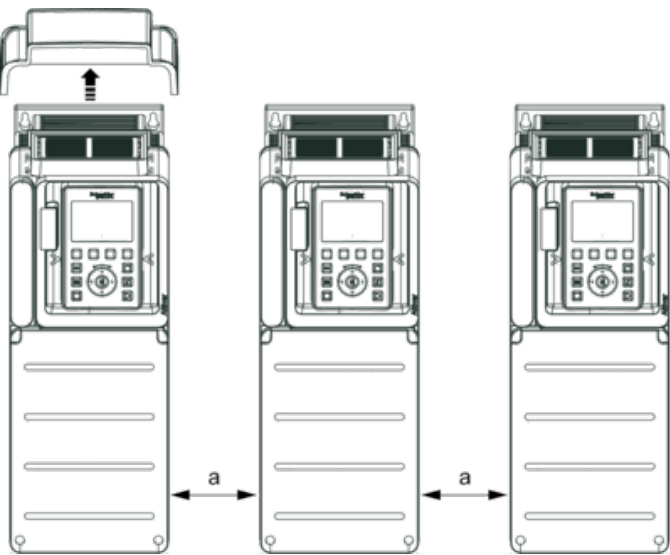
Mounting Type C: Individual IP20
