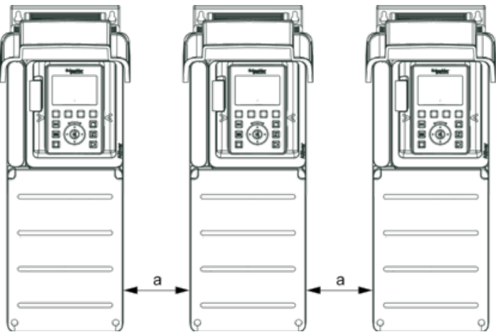
Mounting Type A: Individual IP21
