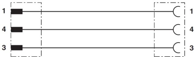
Contact assignment the M12 connector
