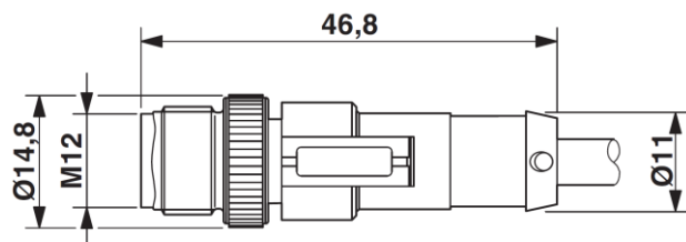
Dimensional drawing
