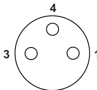
M8-jack, 3-pins, A-coding
