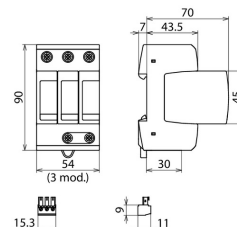
Dimension drawing DG MP TNC ACI 275 FM
