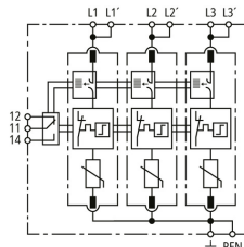
Basic circuit diagram DG MP TNC ACI 275 FM
