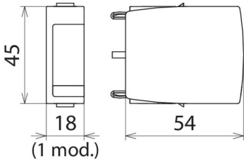
Dimension drawing DG MOD ACI 275
