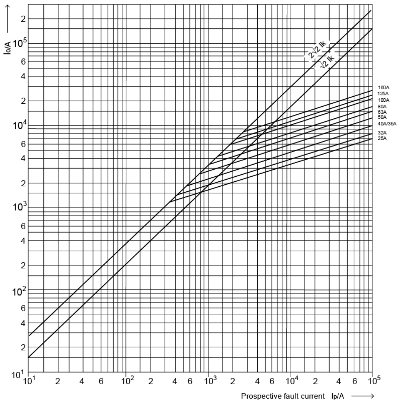
Cut-off characteristics
