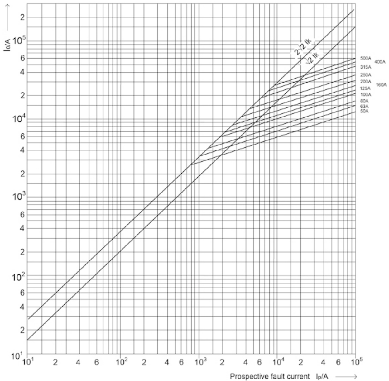
Cut-off characteristics
