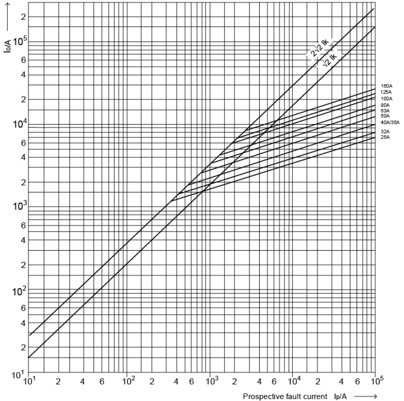
Cut-off characteristics
