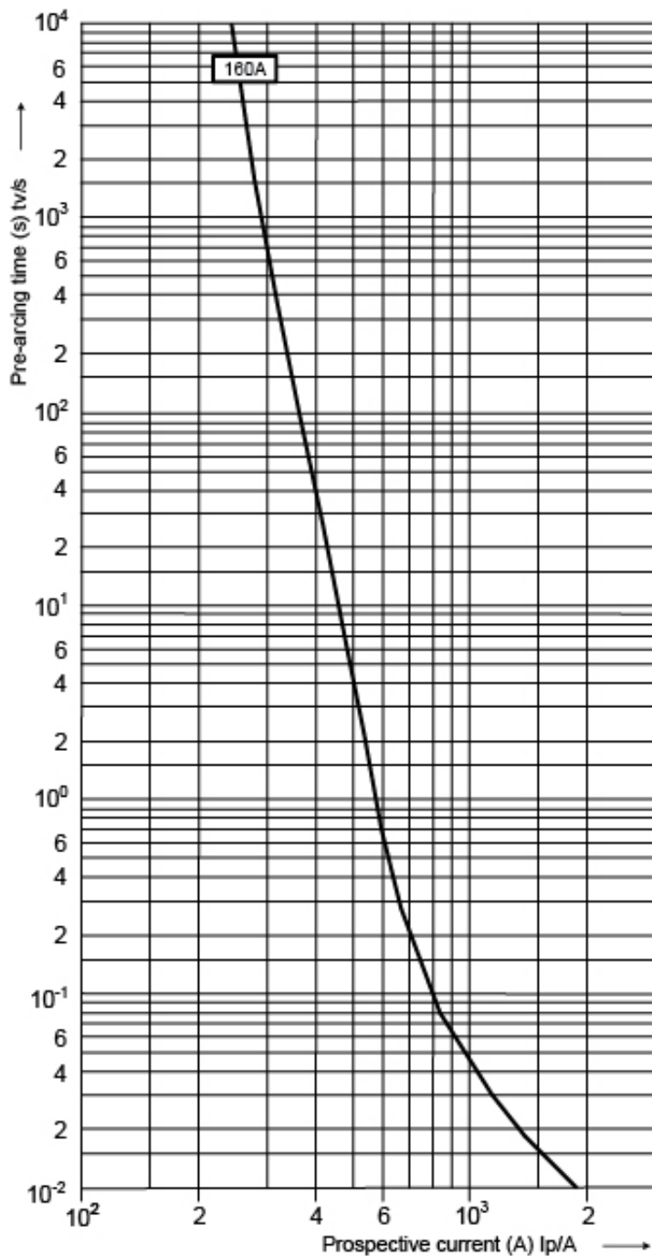
Time-current characteristics NH000L
