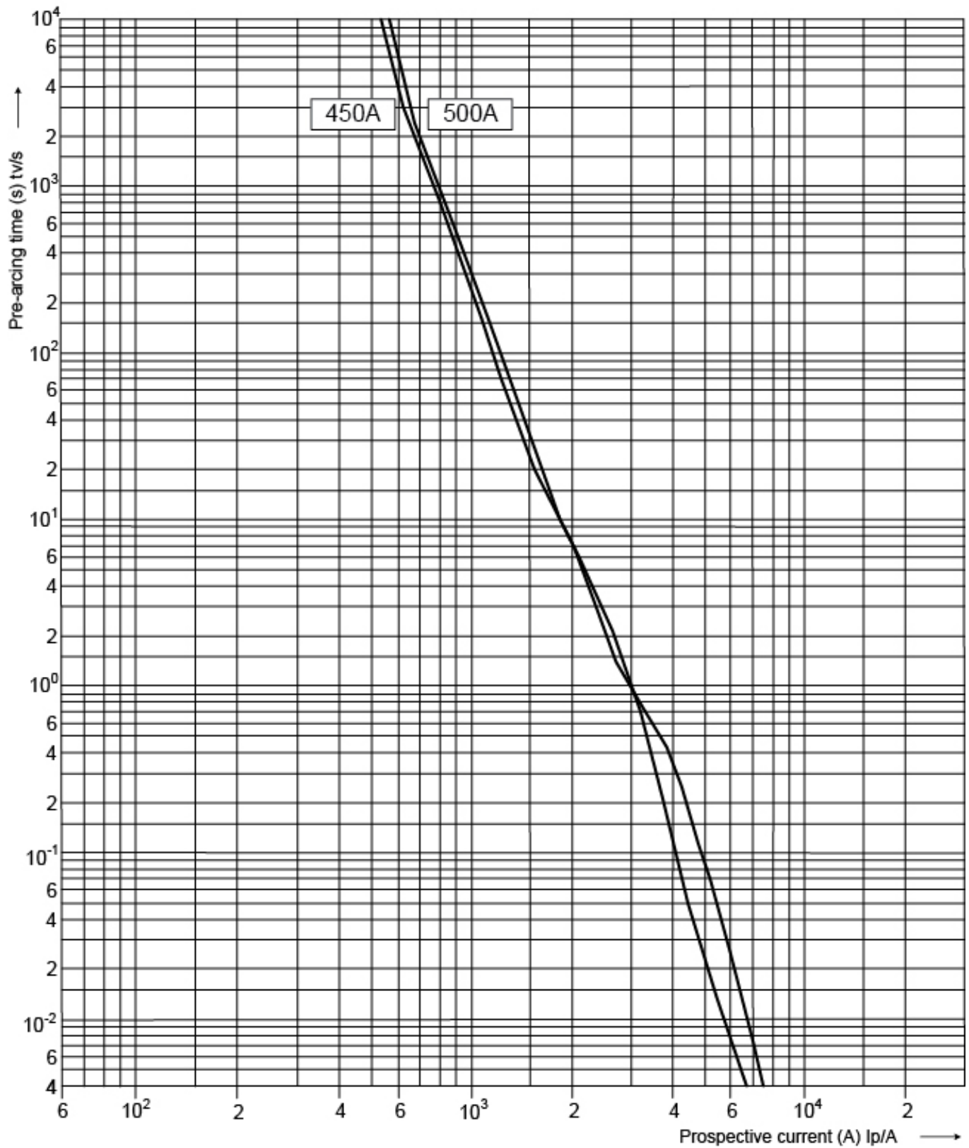
Time-current characteristics
