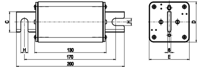
S170 screw contact
