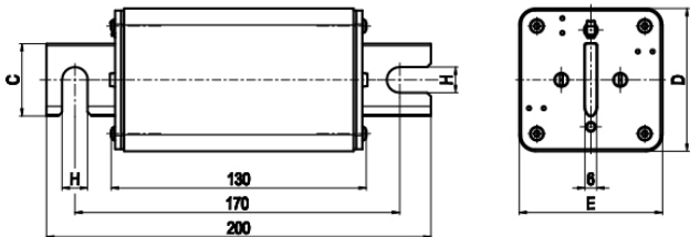
S170 screw contact
